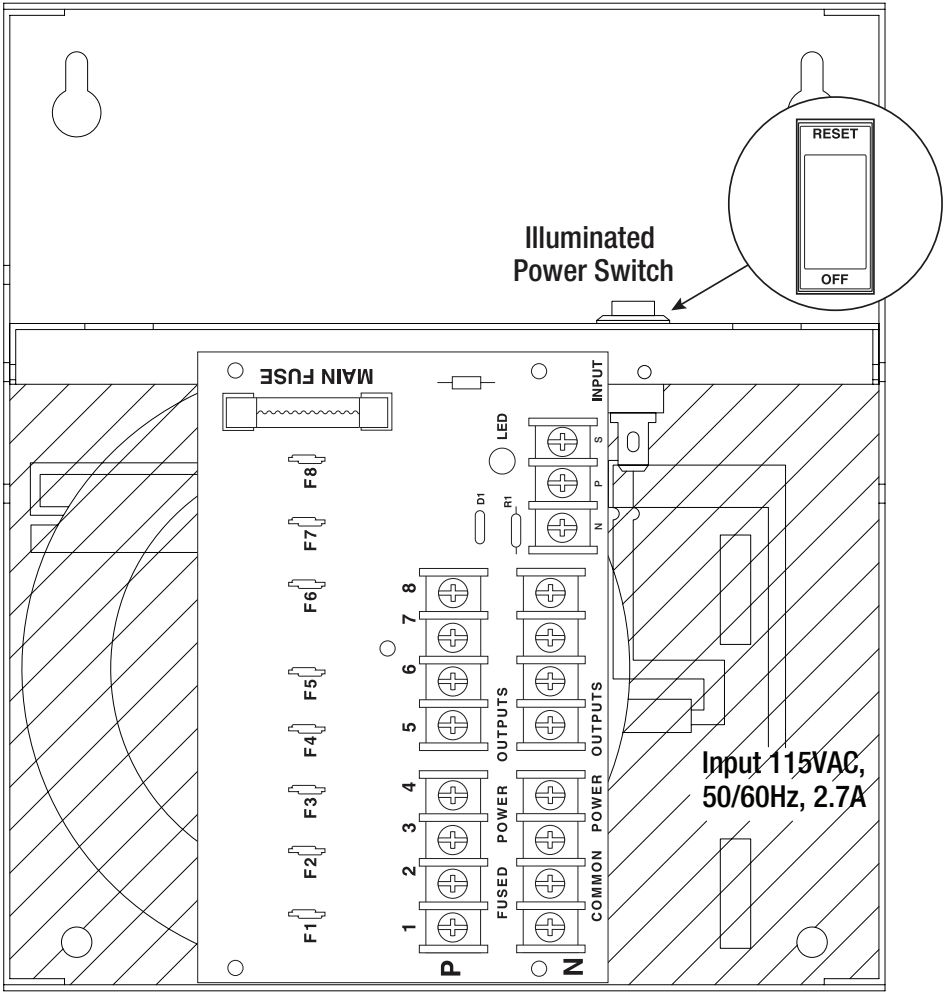
Fig. 4 - AL168300CBM
