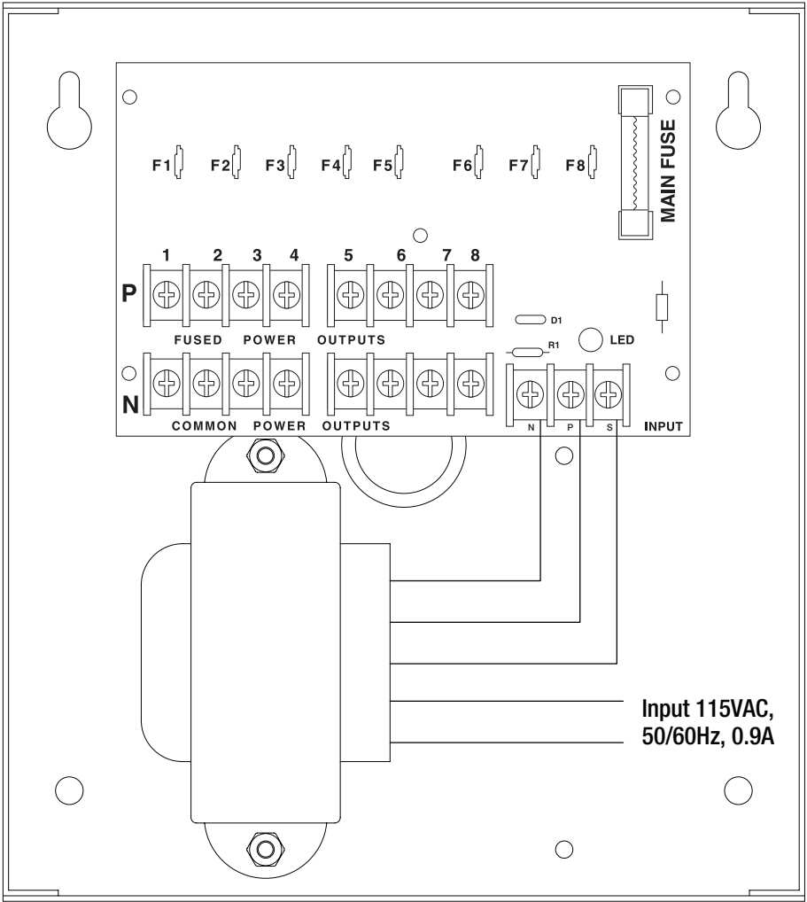
Fig. 1 - AL168CB
