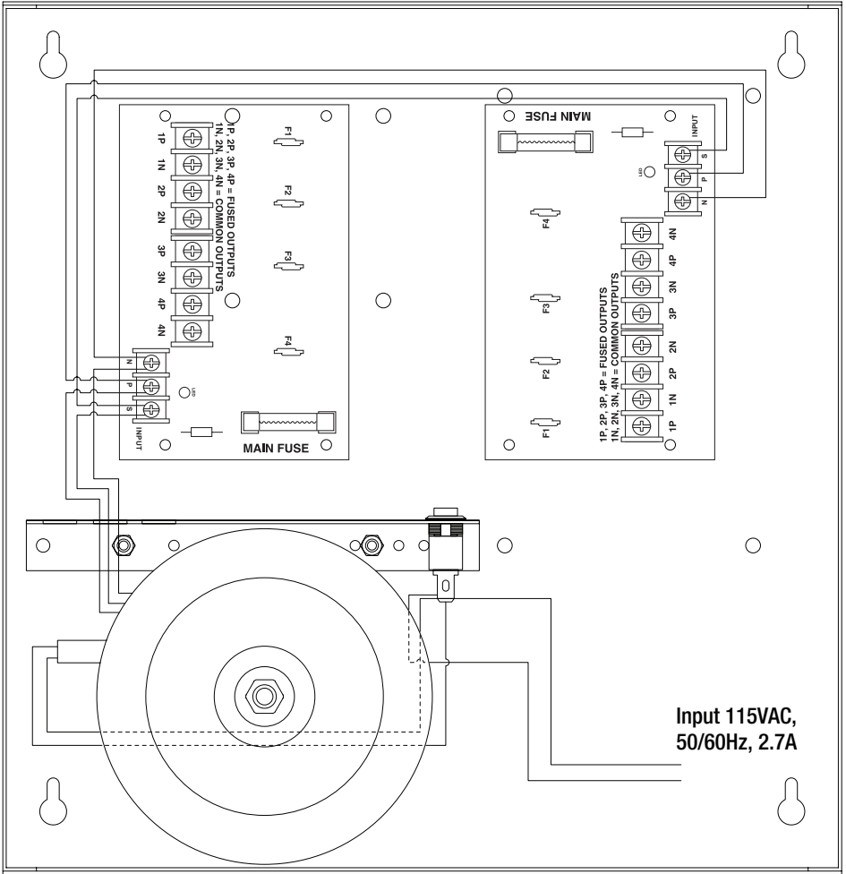
Fig. 3 - AL168300CB
