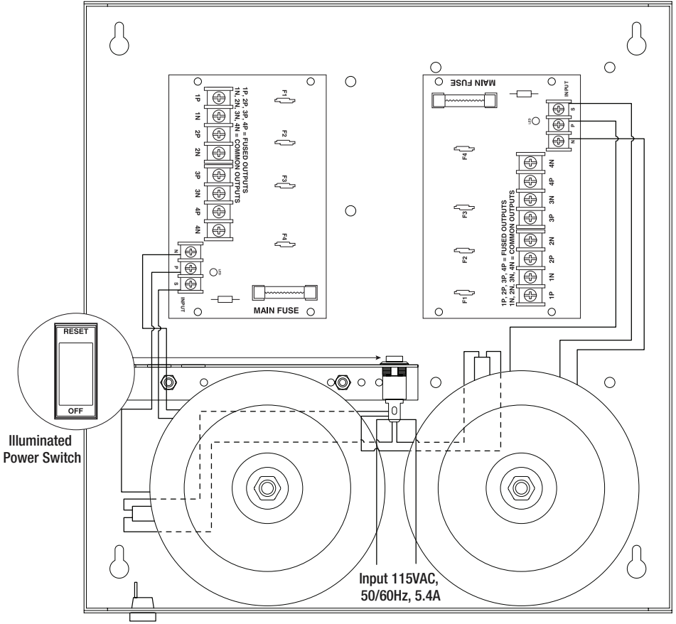
Fig. 5 - AL168600CB
