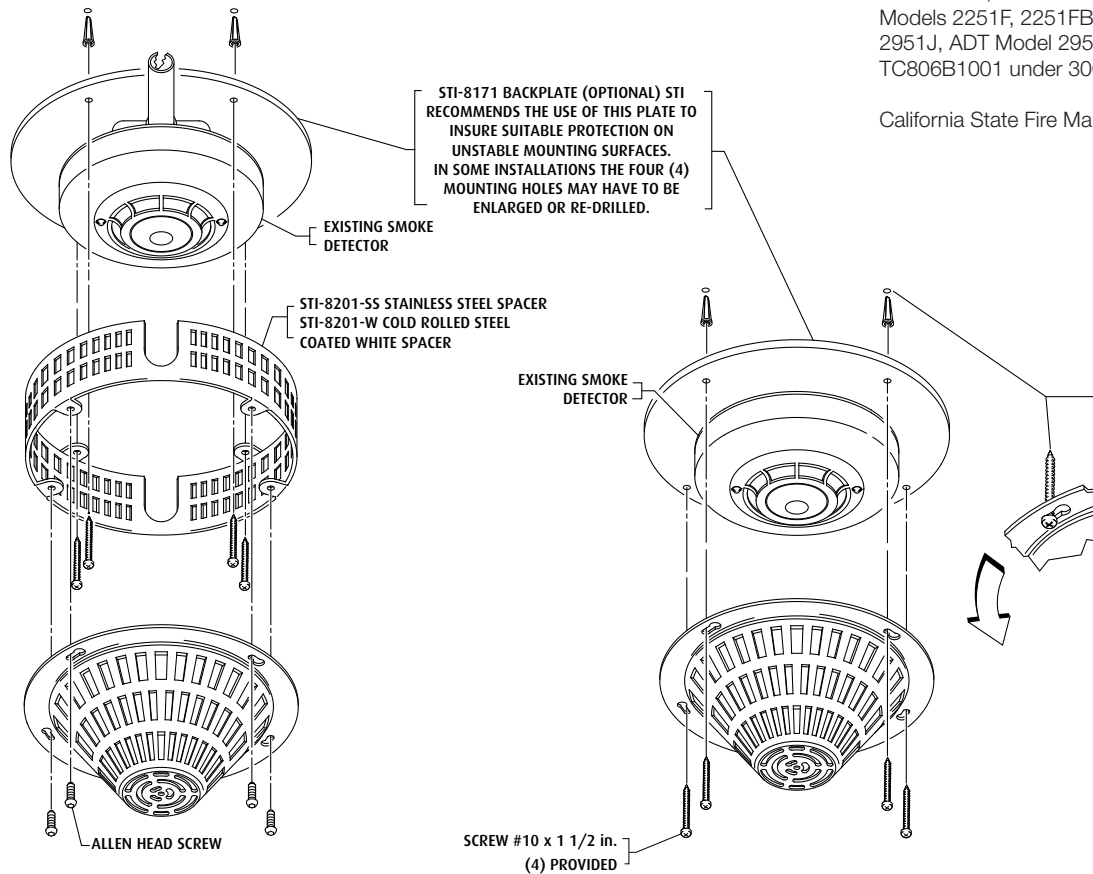
SURFACE MOUNT INSTALLATION
