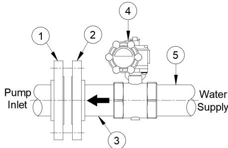
2" (DN50) Pump Skid Water Supply Connection Kit, P/N 73-0170
