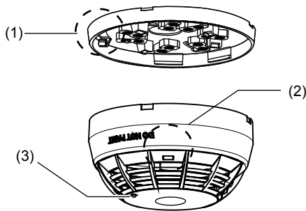
Figure 2: V-PCOS features
