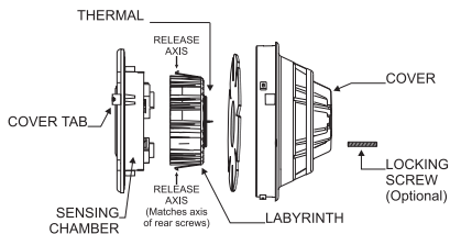
Figure 2 Disassembling of Photochamber
