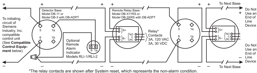
Figure 1 Installation and Wiring Diagram
