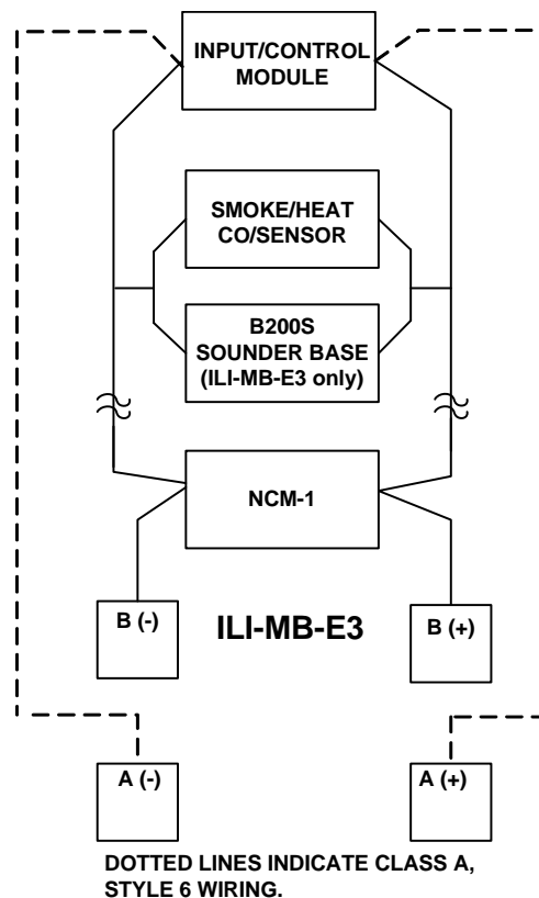
Figure 3.1.1 Signaling Line Circuits
