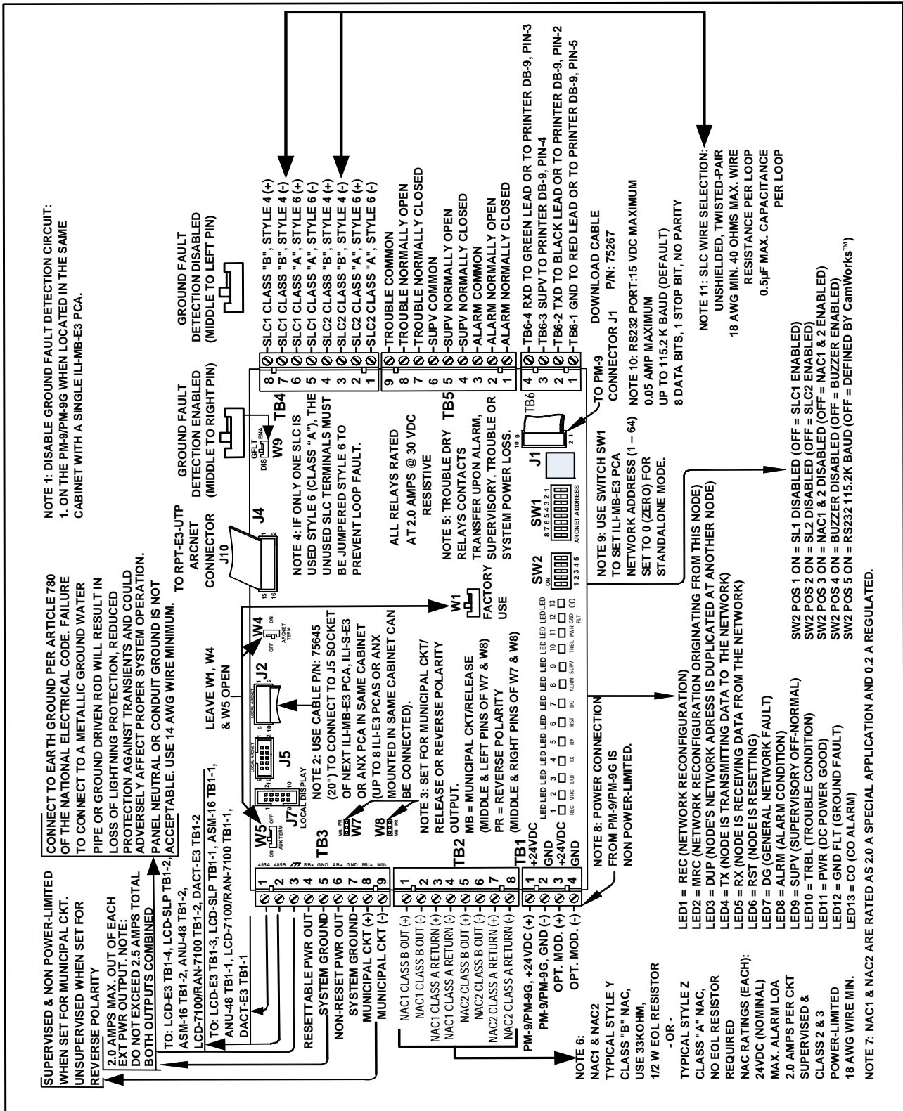
Figure 3.5.3.2.1 ILI-MB-E3 (Second Generation) Wiring Diagram
