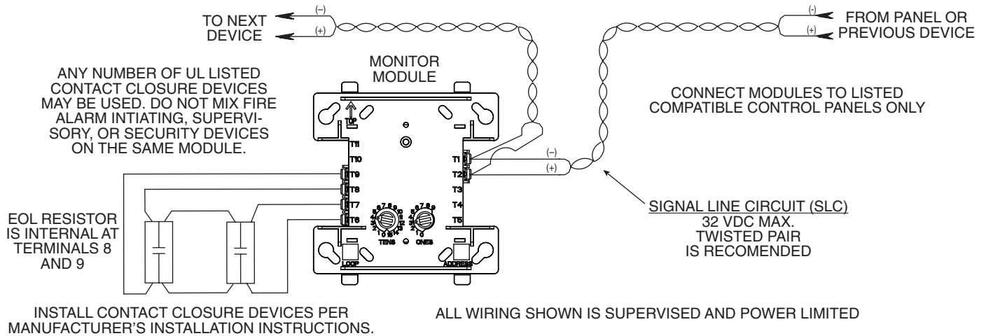
FIGURE 4. TYPICAL 4-WIRE FAULT TOLERANT INITIATING CIRCUIT CONFIGURATION, NFPA STYLE D:
