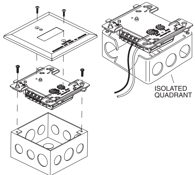
FIGURE 2. MODULE MOUNTING:
