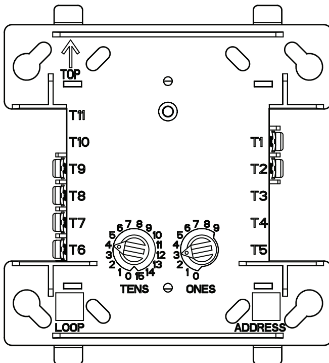
FIGURE 1. CONTROL AND INDICATORS:
