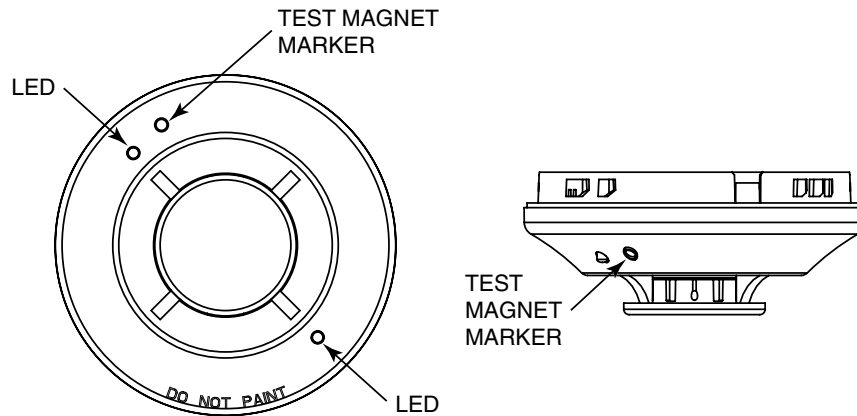
Figure 3. Views showing position of test magnet.
