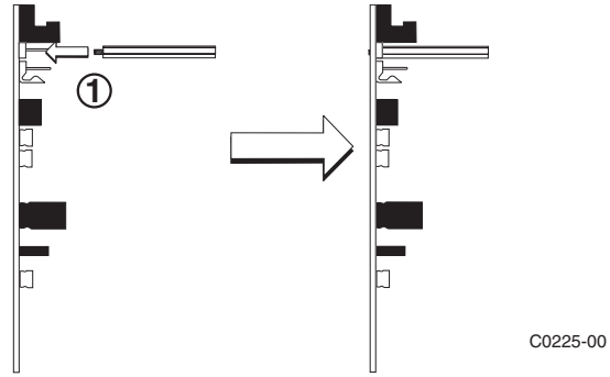
Figure 4a: Installation of IDP-Monitor-10 module in a rear chassis position, method two
