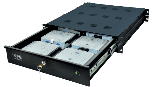
Trove1V1R with six (6) HID VertX® (or Aero™) access controllers
