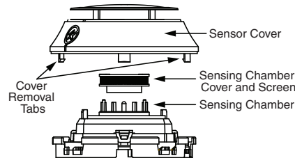
FIGURE 4: CLEANING THE PHOTO DETECTOR
