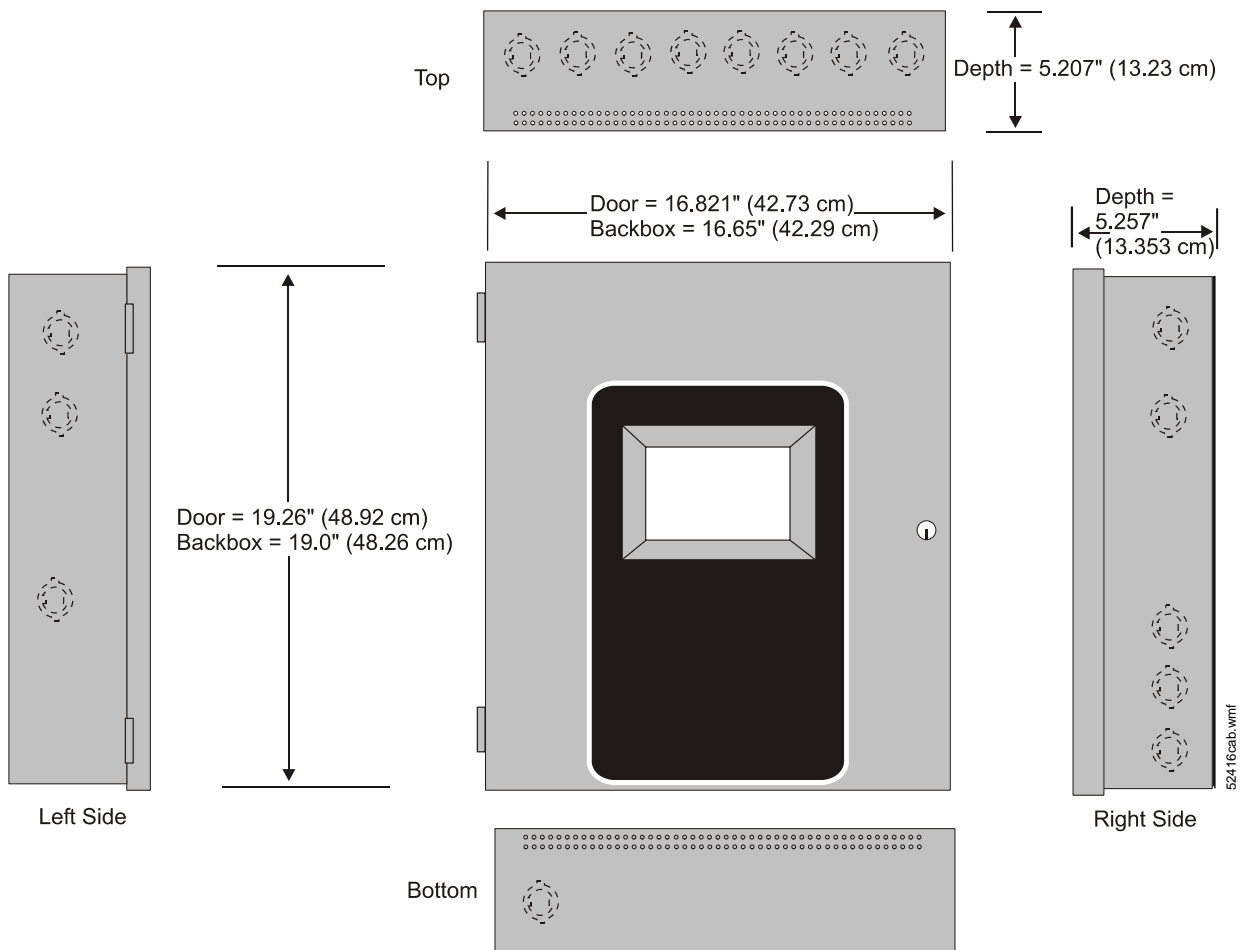
Cabinet Measurements
