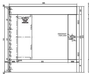
(FRONT VIEW) (SIDE VIEW) CABINET DOOR
