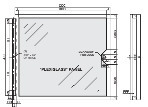
(FRONT VIEW) (SIDE VIEW) PLEXIGLASS DOOR
