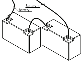
Battery connection (non-power limited). Use two (2) 12V batteries connected in series.
