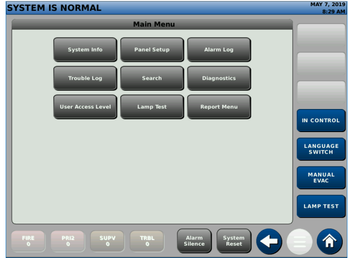
Figure 4: Main Menu
