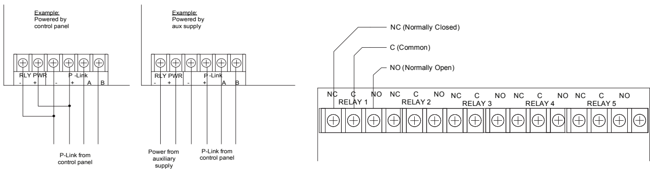
Figure 29. RLY-5 Wiring to Control Panel / Auxiliary Power Supply & RLY-5 Normally Open / Normally Closed Contacts
