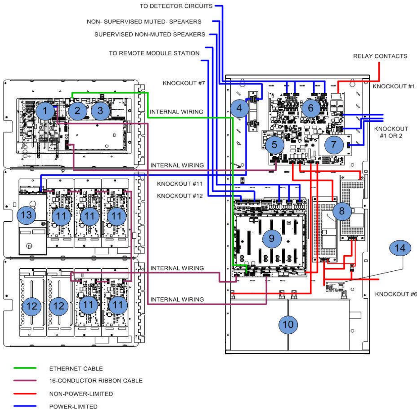
Figure 3: Module Location in 3HU Enclosure and Recommended Wire Routing
