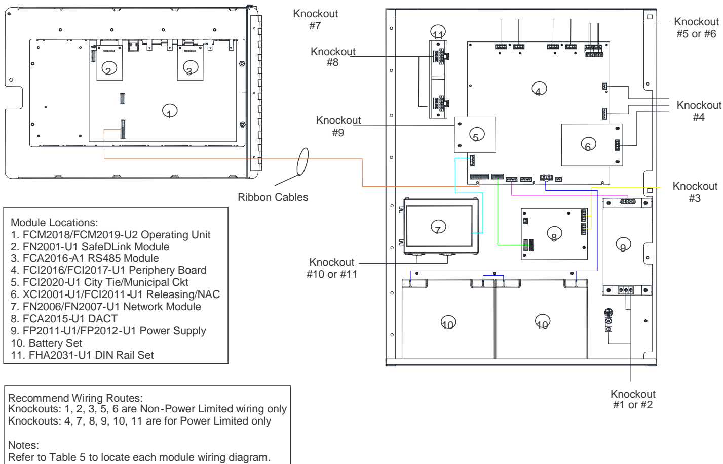
Figure 1: Module Location in 2HU Enclosure and Recommended Wire Routing
