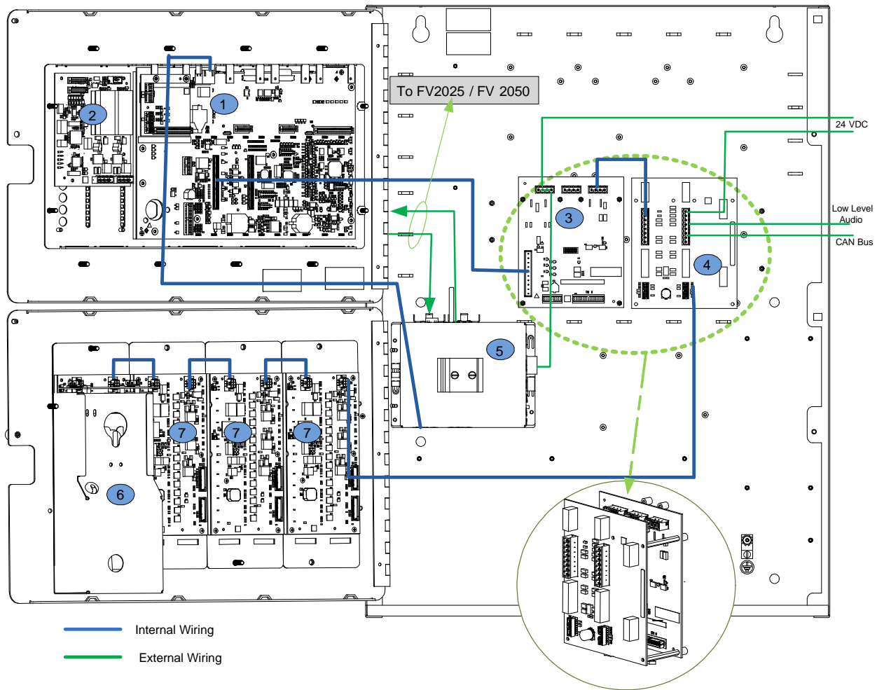
Figure 5: Module Location for 2HU Enclosure (Remote Station) and Recommend Wire Routing
