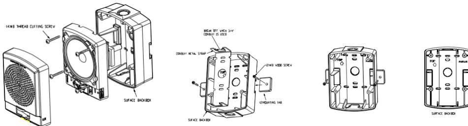
Figure 6: Surface Backbox Mounting
