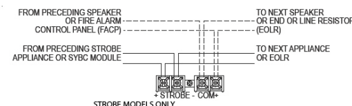
Figure 1: Strobe Wiring
