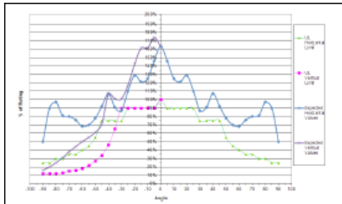
Figure 5: Expected Candela Ratings
