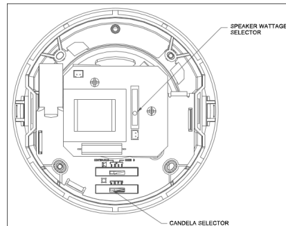
Figure 5: Speaker Switch and Candela Selectors
