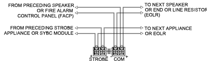
Figure 1 LED Strobe Wiring
