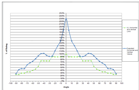
Figure 4: LED Ceiling Expected Candela Ratings
