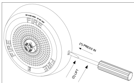
Figure 8: Removing a Speaker or Speaker Strobe
