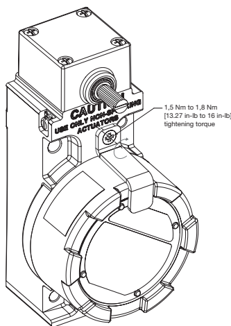
FIGURE 10. WIRING INSTRUCTIONS
