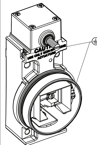
FIGURE 11. WIRING INSTRUCTIONS
