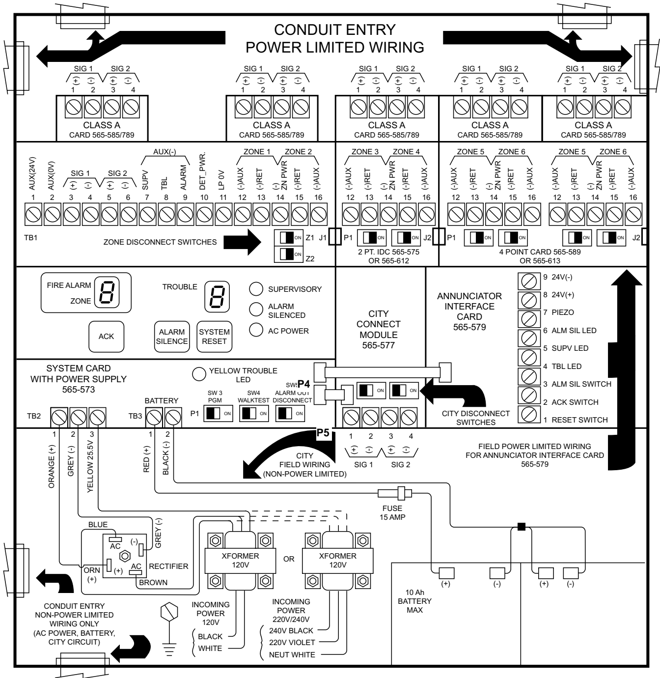
Figure 1. 4004 System Diagram
