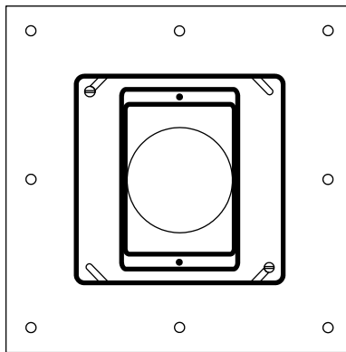
Figure 17. The SIGA-DMP Duct Detector Mounting Plate for DS-PS Smoke Detector
