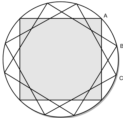
Figure 2. Heat Detector's Circle of Coverage
