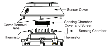
FIGURE 4. CLEANING THE PHOTO/HEAT DETECTOR
