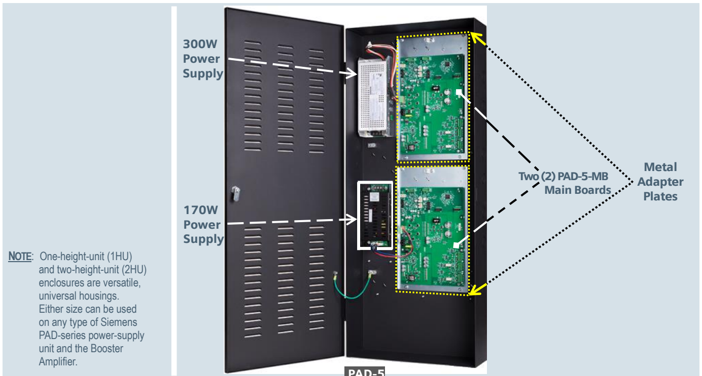
Typical configuration of two (2) main boards mounted in a two-height-unit (2HU) enclosure
