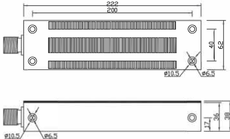
Magnetic lock dimension drawing
