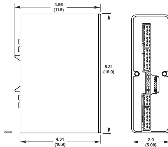
Figure 6—Dimensions of the ASM Module in Inches (Centimeters)
