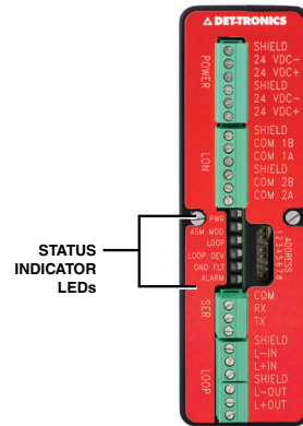
Figure 5—Location of LED Indicators
