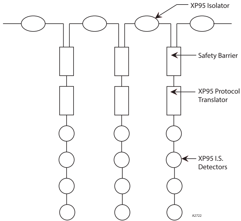
Figure 9—XP95 Wiring Schematic
