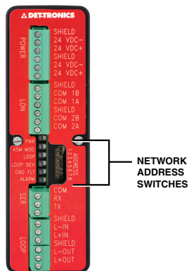
Figure 8—Location of Network Address Switches
