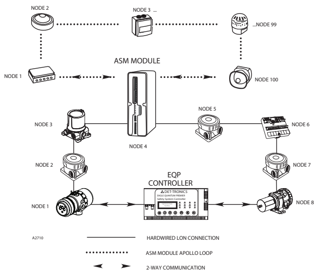
Figure 1—EQP LON with ASM Module Communication
