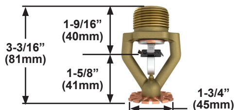
Figure 2: ESFR Pendent Sprinkler VK514 Dimensions
