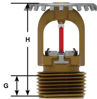
Figure – 2: Dimensions
