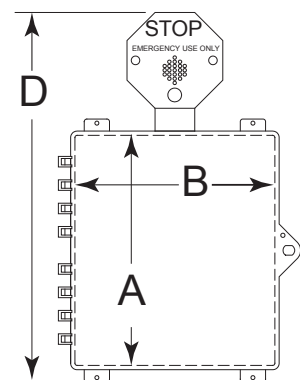
FRONT VIEW for models with Audible Siren Alarm
