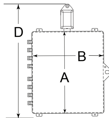
FRONT VIEW for models with Strobe/Siren Alarm
