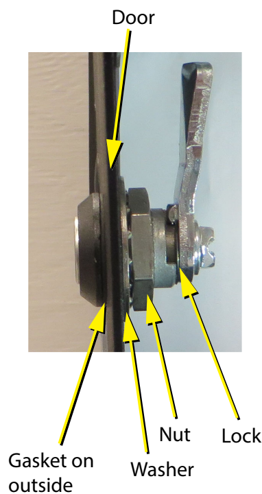
Figure 2 Lockset
