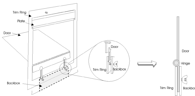
Door Installation
