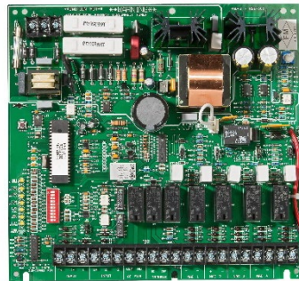
Model PAD-3-MB Main Board
