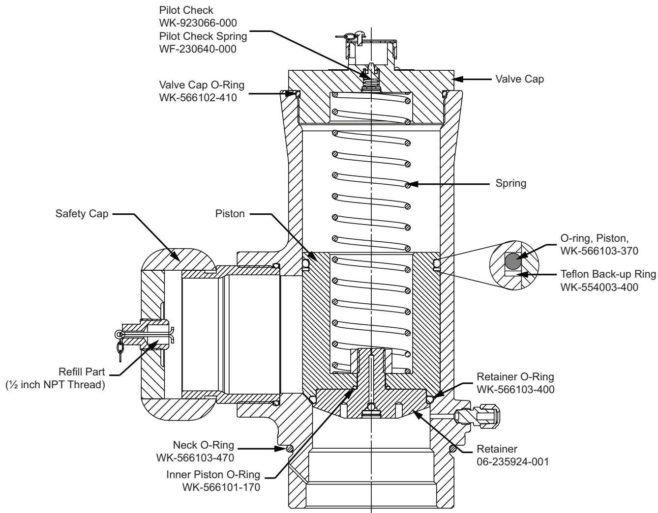
Figure 1. 3-inch Valve Assembly
