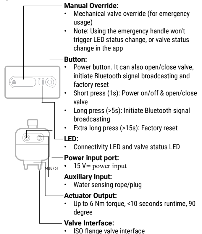
Fig. 2. Components.
