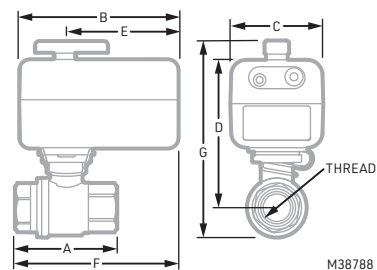
Fig. 7. Dimension diagram.
