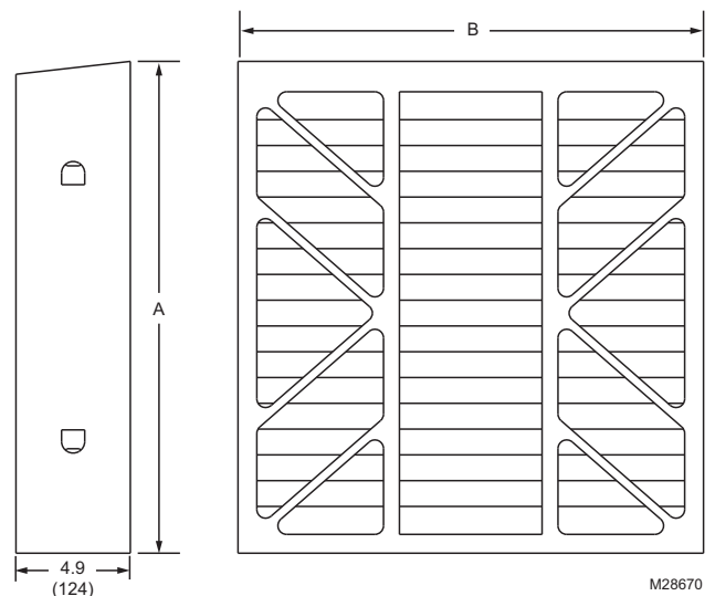
Fig. 1. Dimensions in in. (mm) (see Table 1).
