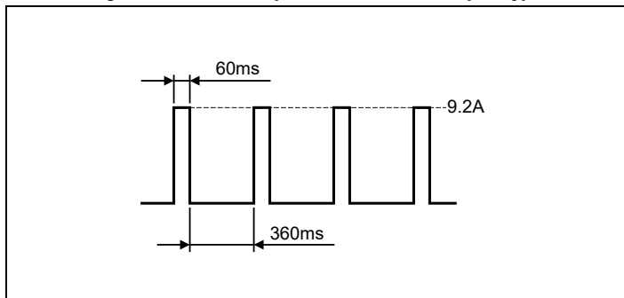
Fig. 6-2 Intermittent operation at shorted output, typ.
