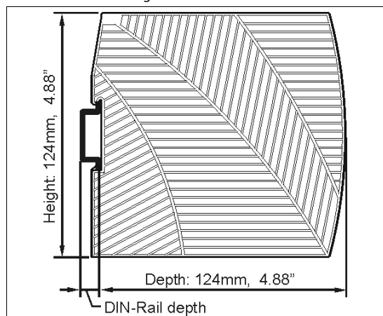
Fig. 21-2 Side view
