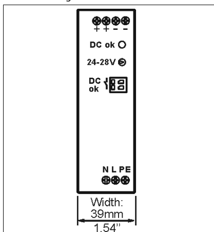
Fig. 21-1 Front view
