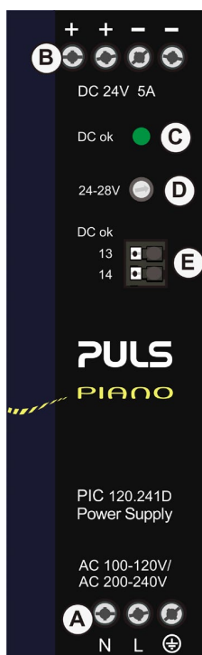
Fig. 11-1 Front side
