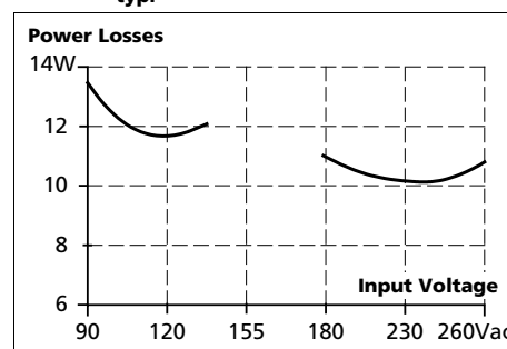
Fig. 9-4 Losses vs. input voltage at 24V, 5A, typ.
