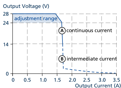
Fig. 6-1: Output voltage vs. output current, typ.
