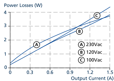
Fig. 8-2: Losses vs. output current at 24V, typ.
