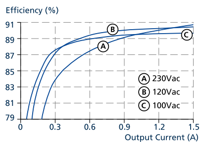
Fig. 8-1: Efficiency vs. output current at 24V, typ.
