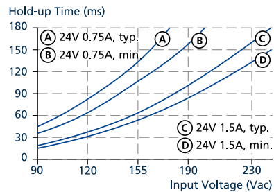
Fig. 7-1: Hold-up time vs. input voltage
