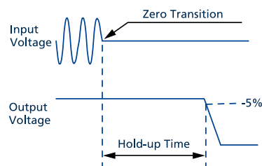
Fig. 7-2: Shut-down behaviour, definitions
