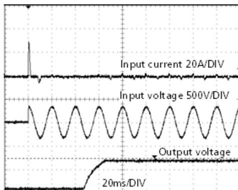
Fig. 5-3: Typical turn-on behavior at 230Vac and 25°C ambient
