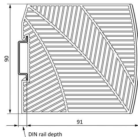
Fig. 20-2: Side view
