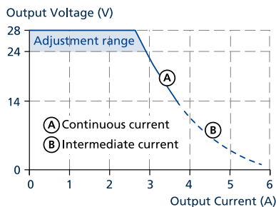
Fig. 6-1: Output voltage vs. output current, typ.
