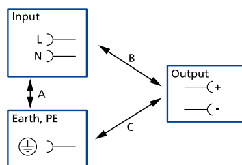
Fig. 17-1: Dielectric strength
