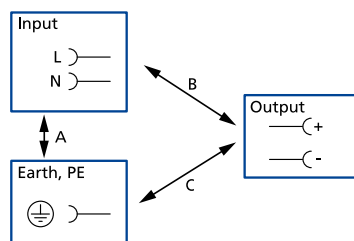
Fig. 17-1: Dielectric strength
