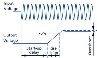
Fig. 3-2: Turn-on behavior, definitions
