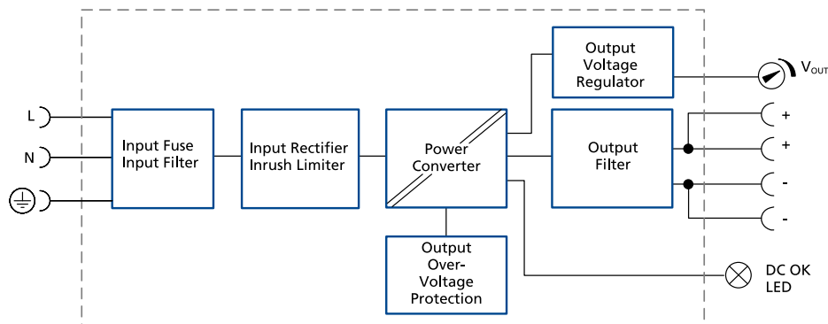
Fig. 11-1: Functional diagram
