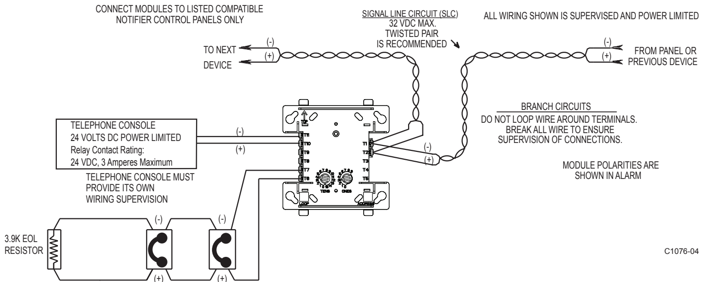
Figure 3. Typical circuit configuration, NFPA Class B:
