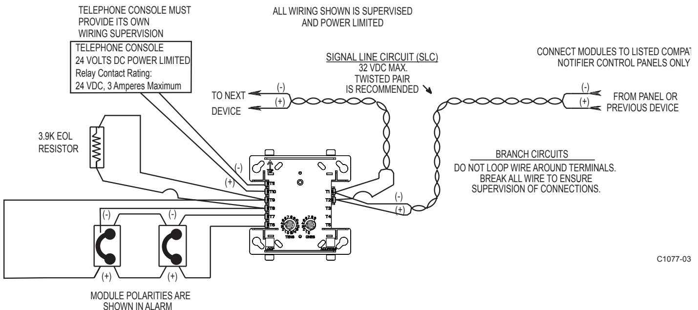
Figure 4. Typical fault tolerant circuit configuration, NFPA Class A:
