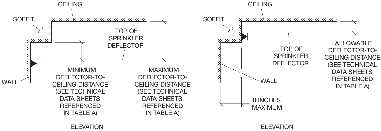
FIGURE 2 (PART 2 OF 2) POSITION OF HORIZONTAL SIDEWALL SPRINKLERS WITH RESPECT TO OBSTRUCTIONS ALONG A WALL TO AVOID OBSTRUCTION TO WATER DISTRIBUTION
