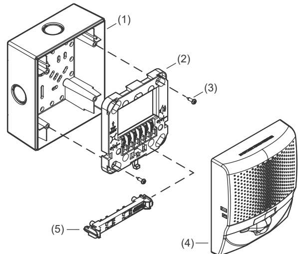
Figure 4: Typical surface box mounting
