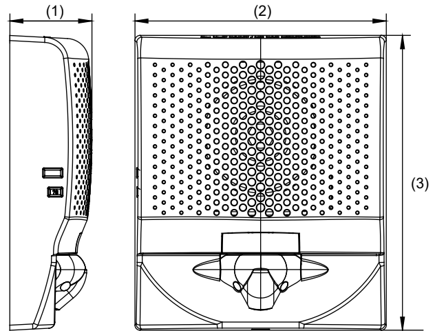
Figure 9: Dimensions
