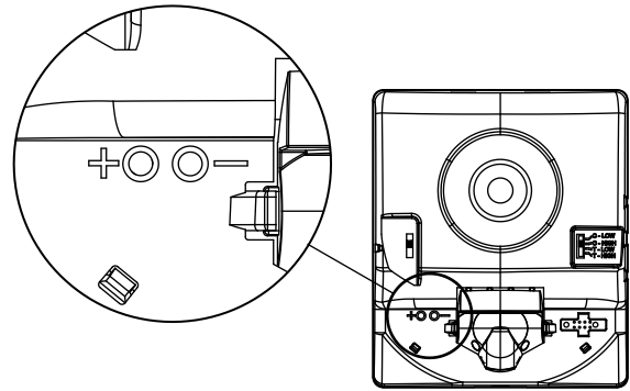
Figure 7: Test points
