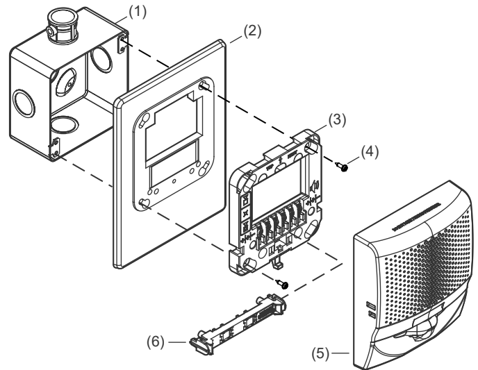
Figure 3: Typical electrical box mounting
