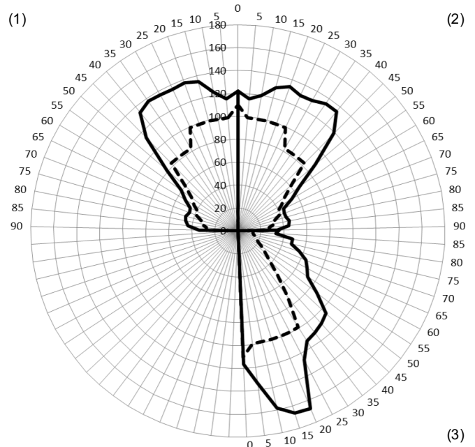
Figure 8: 110 cd light distribution
