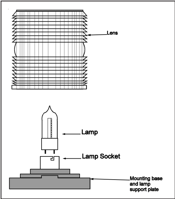
Figure 3. Lamp Replacement
