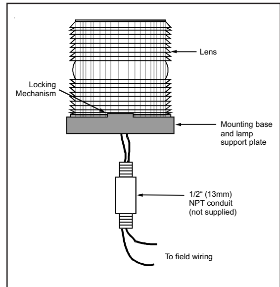
Figure 1. Conduit Mounting
