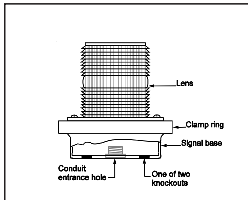
Figure 2. Catalog Series 50 and 50SIN Flashing Lights
