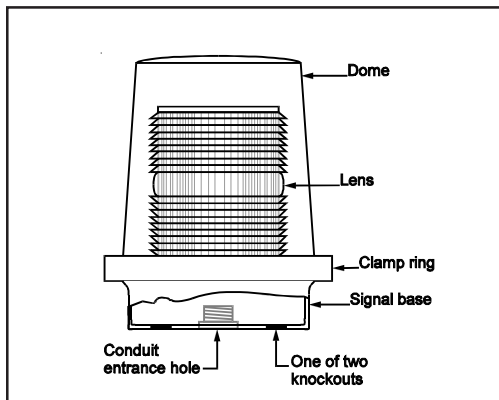
Figure 1. Catalog Series 49 Flashing Lights
