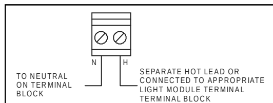
Figure 2. Wiring the Tone Module
