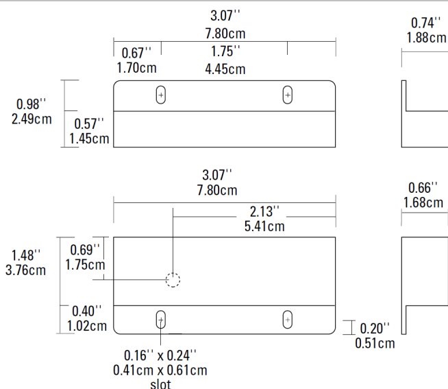
Figure 1: Dimensions
