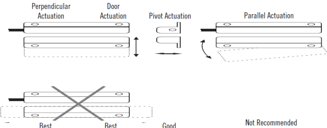
Figure 3: Mounting configurations
