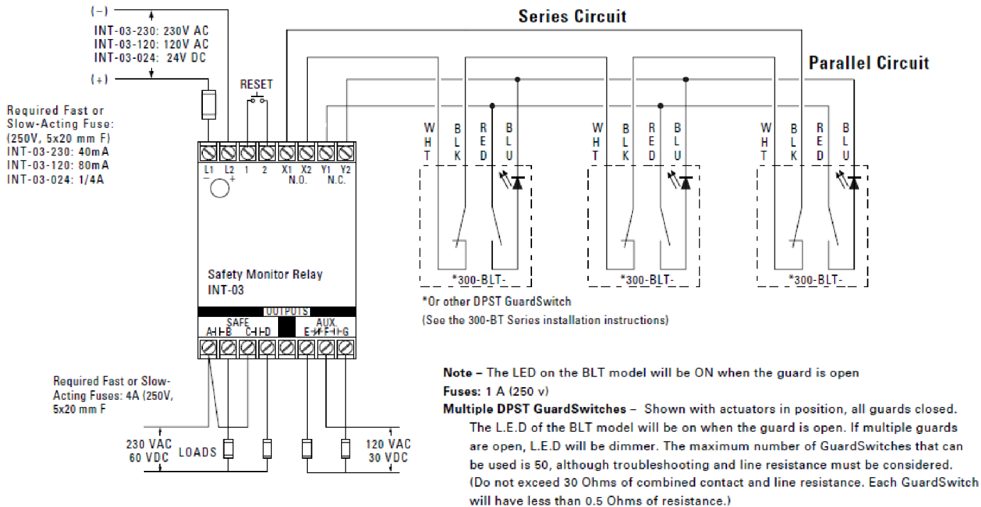
Figure 5: Wiring for category 3
