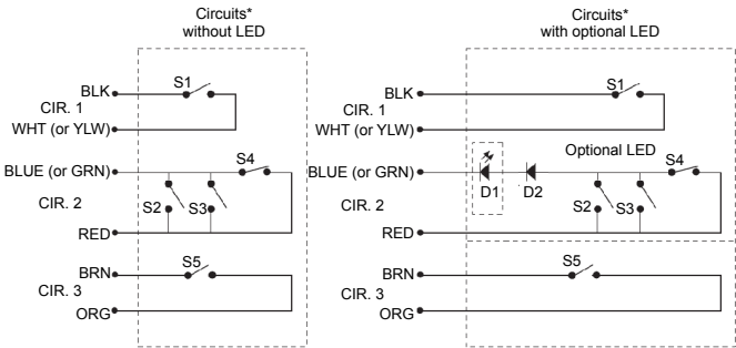
Figure 4: Circuits
