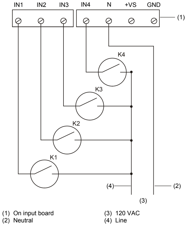
Figure 13: Connection from a PLC to input board, 120 V input board. See Table 5
