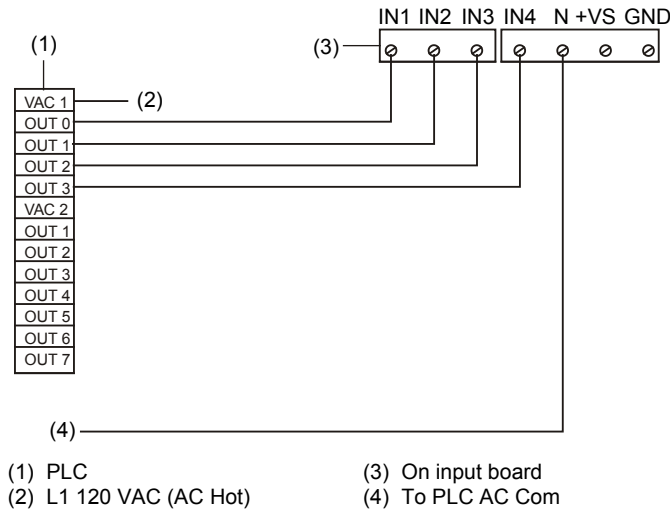
Figure 13: Connection from a PLC to input board, 120 V input board. See Table 5
