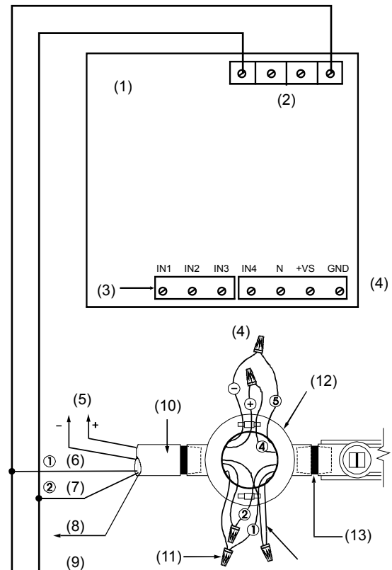
Figure 4: Wiring diagram
